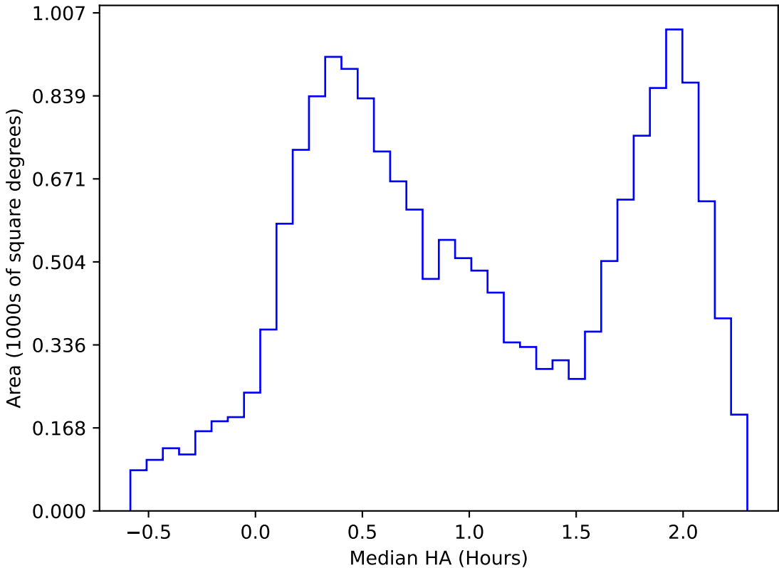
roll_uniform_eh_acc0.2_mjdp0_v3.4_10yrs WFD i band: Median HA
