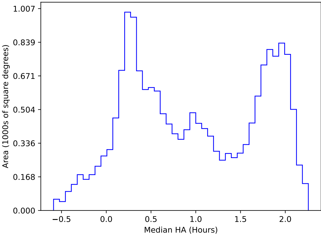
roll_uniform_eh_acc0.2_mjdp0_v3.4_10yrs WFD all bands: Median HA
