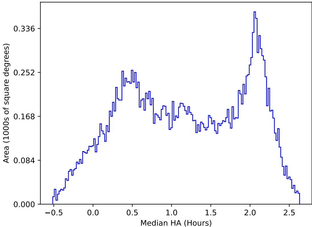
roll_uniform_eh_acc0.2_mjdp0_v3.4_10yrs All sky y band: Median HA
