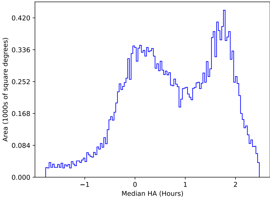
roll_uniform_eh_acc0.2_mjdp0_v3.4_10yrs All sky u band: Median HA
