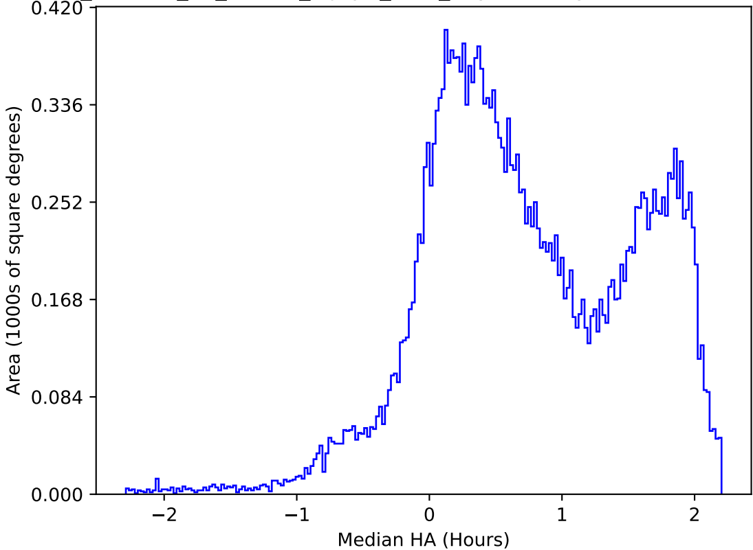
roll_uniform_eh_acc0.2_mjdp0_v3.4_10yrs All sky r band: Median HA
