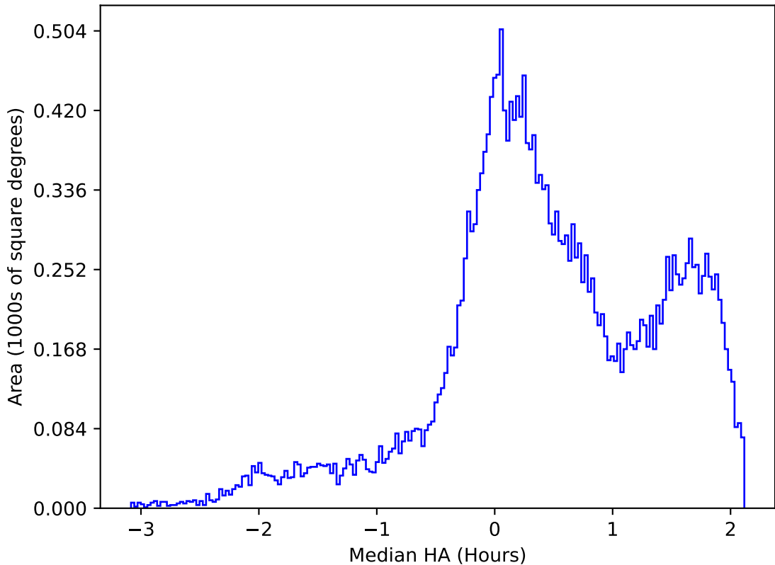
roll_uniform_eh_acc0.2_mjdp0_v3.4_10yrs All sky g band: Median HA
