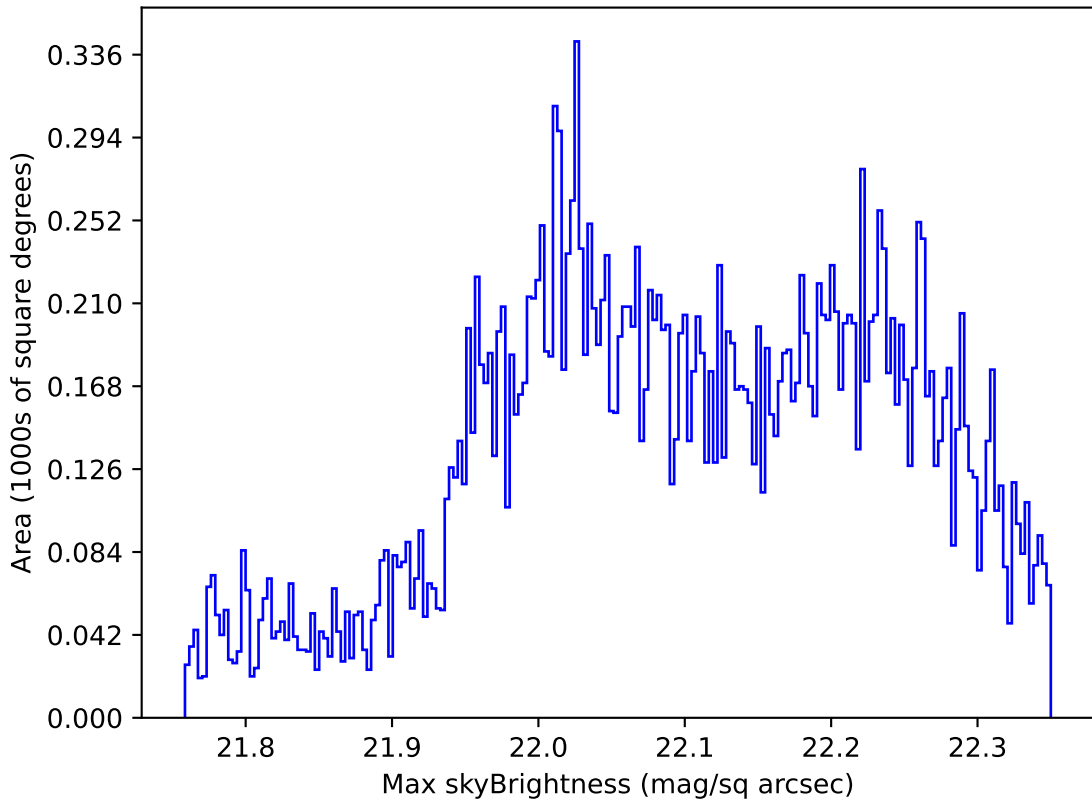
roll_uniform_eh_acc0.2_mjdp0_v3.4_10yrs Yr 1 g band: Max skyBrightness
