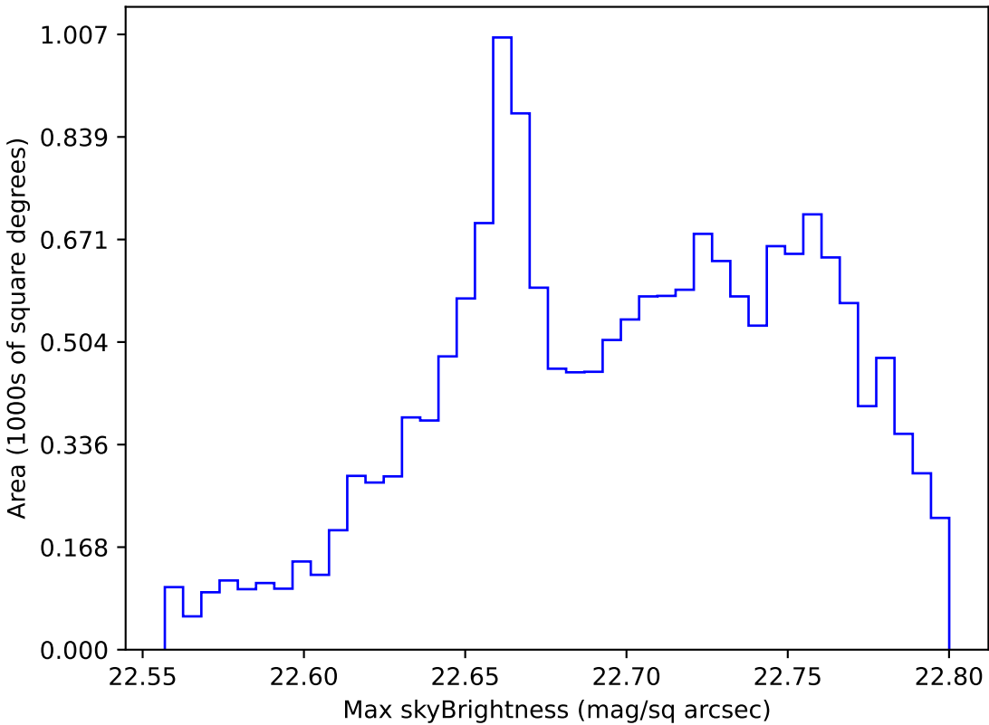
roll_uniform_eh_acc0.2_mjdp0_v3.4_10yrs WFD u band: Max skyBrightness
