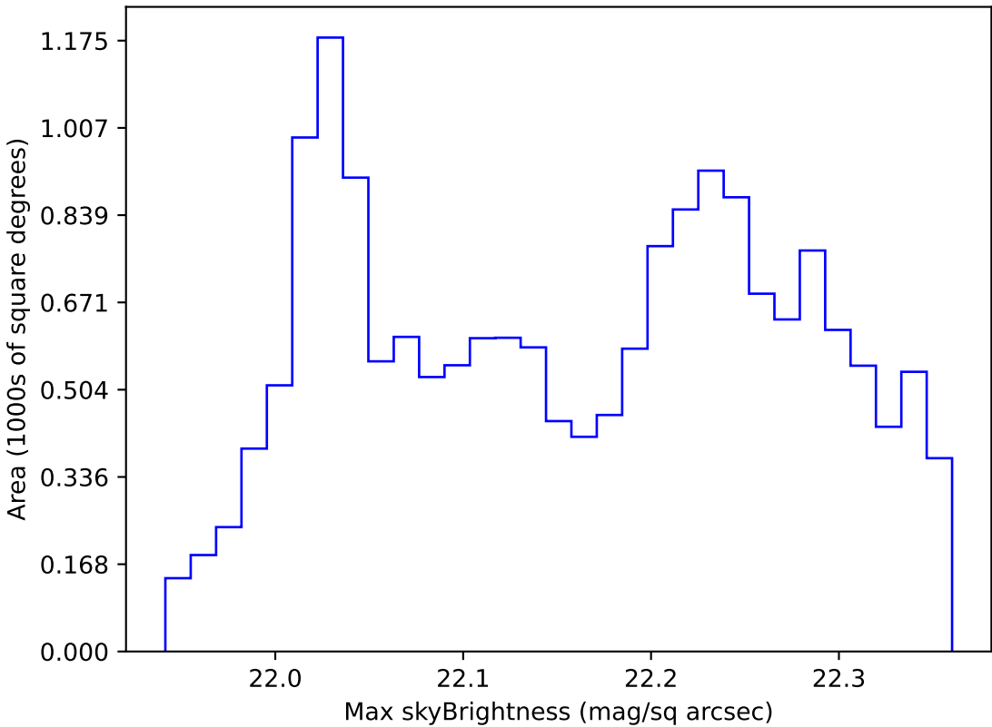
roll_uniform_eh_acc0.2_mjdp0_v3.4_10yrs WFD g band: Max skyBrightness
