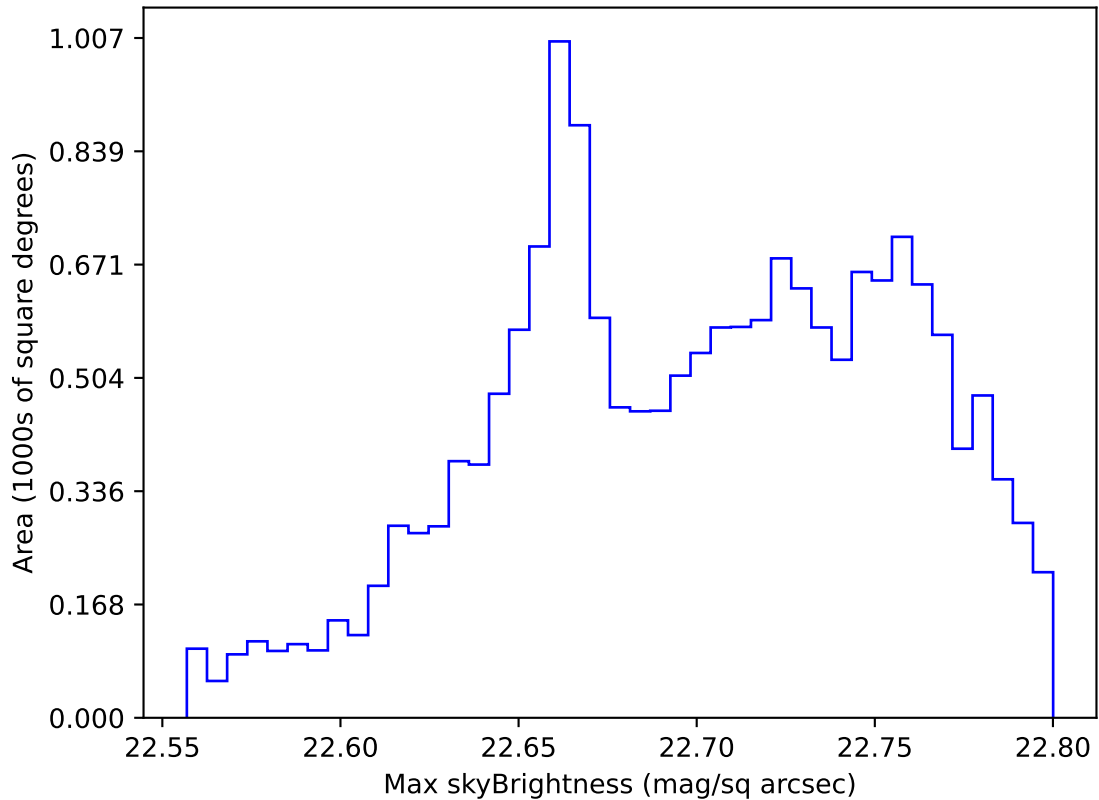
roll_uniform_eh_acc0.2_mjdp0_v3.4_10yrs WFD all bands: Max skyBrightness
