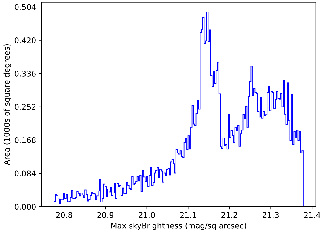
roll_uniform_eh_acc0.2_mjdp0_v3.4_10yrs All sky r band: Max skyBrightness
