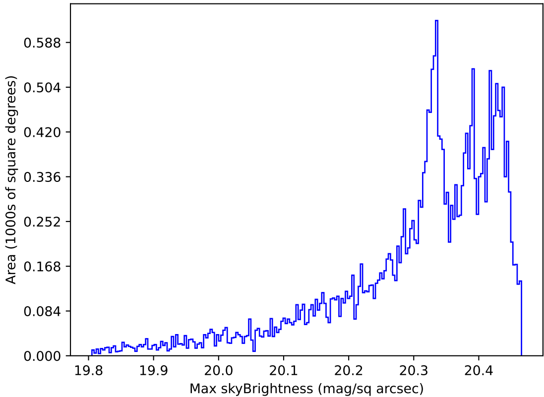
roll_uniform_eh_acc0.2_mjdp0_v3.4_10yrs All sky i band: Max skyBrightness
