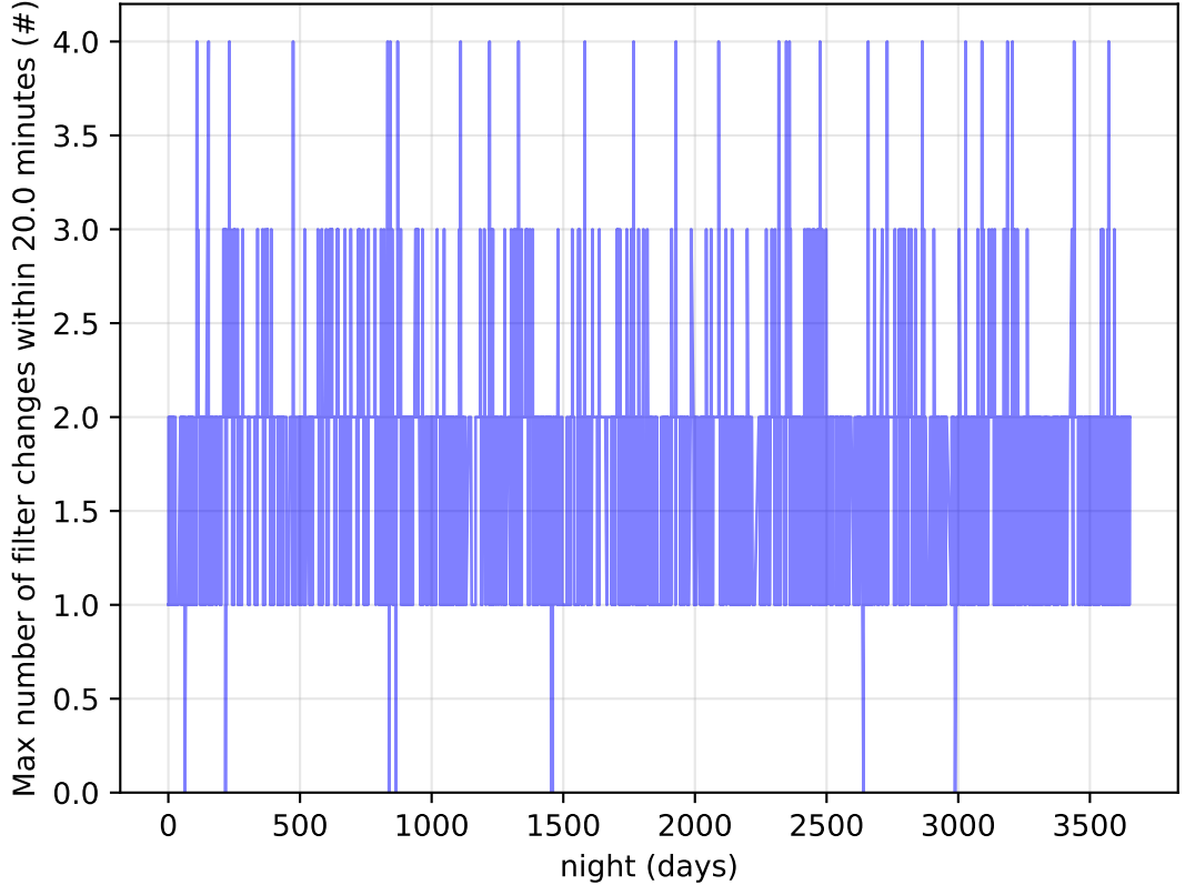
roll_uniform_eh_acc0.2_mjdp0_v3.4_10yrs Per Night: Max number of filter changes within 20.0 minutes
