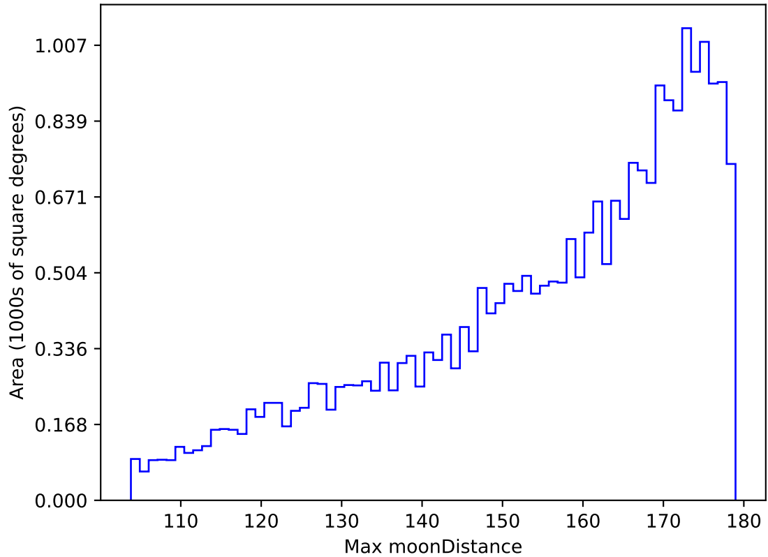
roll_uniform_eh_acc0.2_mjdp0_v3.4_10yrs All sky g band: Max moonDistance
