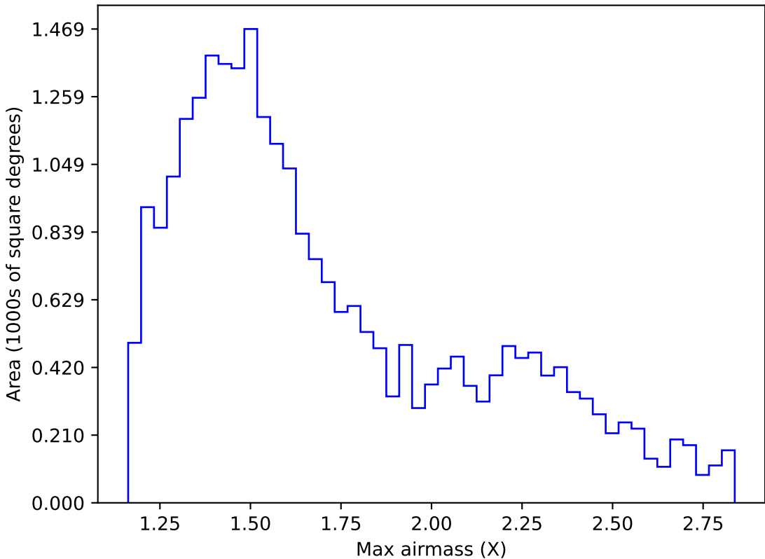
roll_uniform_eh_acc0.2_mjdp0_v3.4_10yrs Yr 1 i band: Max airmass
