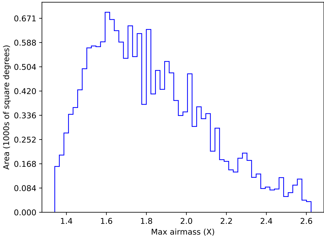
roll_uniform_eh_acc0.2_mjdp0_v3.4_10yrs WFD u band: Max airmass
