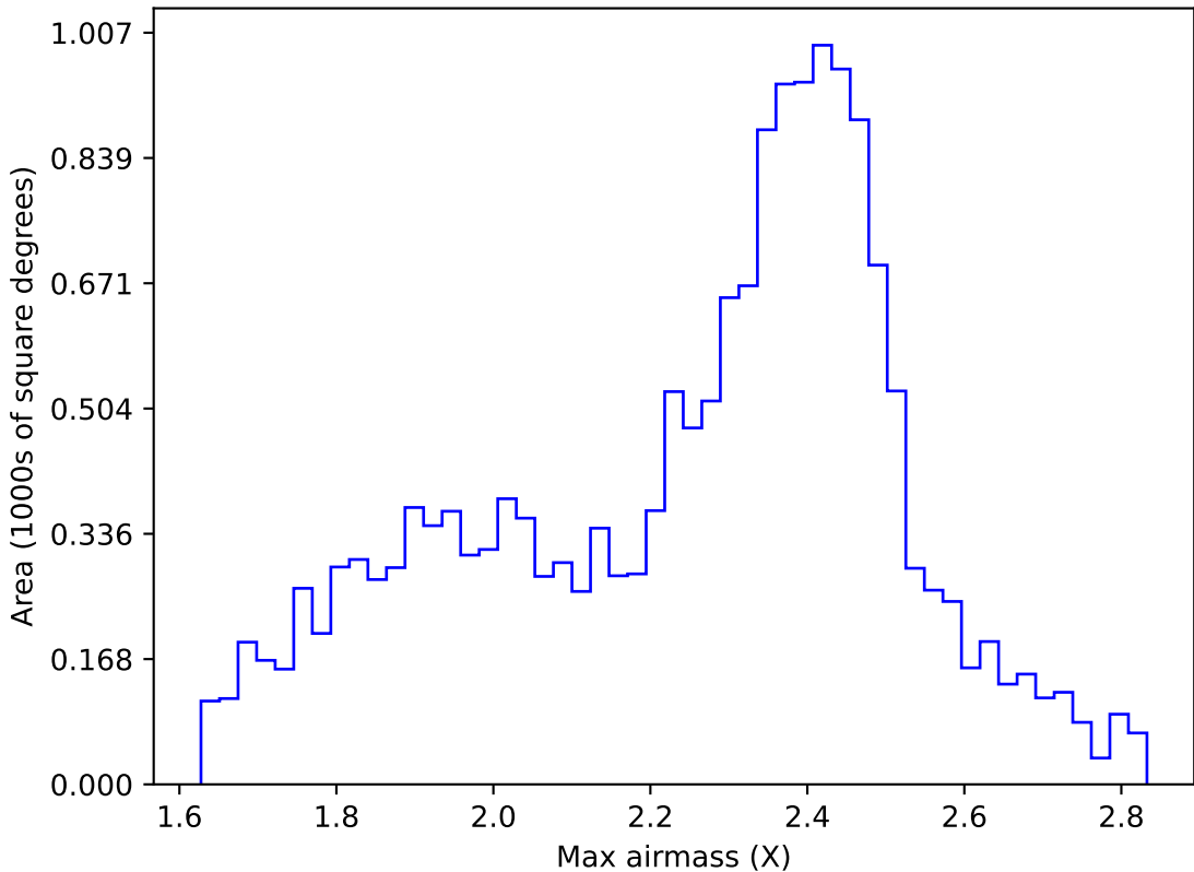
roll_uniform_eh_acc0.2_mjdp0_v3.4_10yrs WFD r band: Max airmass
