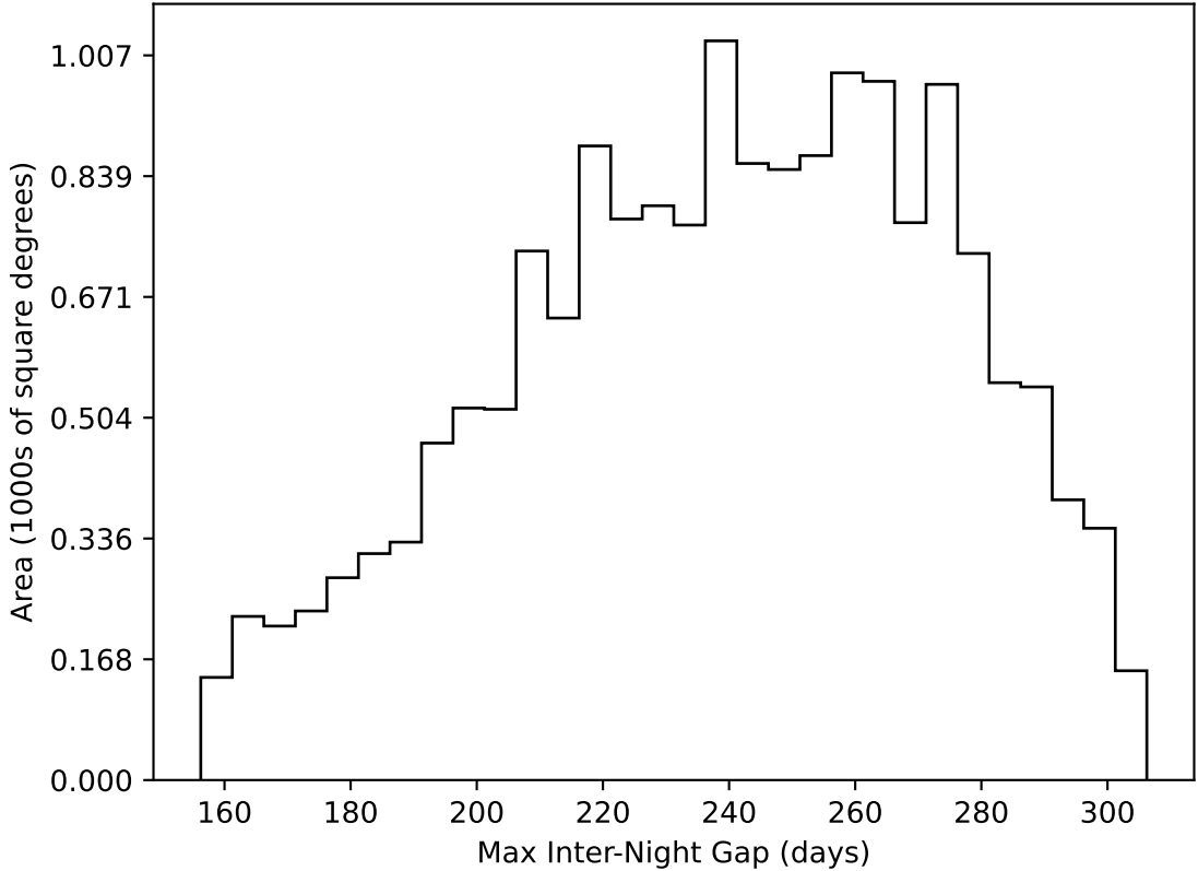
roll_uniform_eh_acc0.2_mjdp0_v3.4_10yrs WFD all bands: Max Inter-Night Gap
