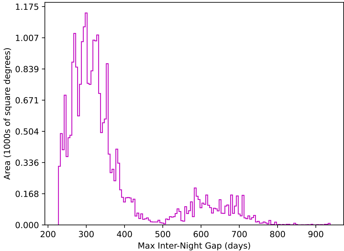
roll_uniform_eh_acc0.2_mjdp0_v3.4_10yrs All sky z band: Max Inter-Night Gap
