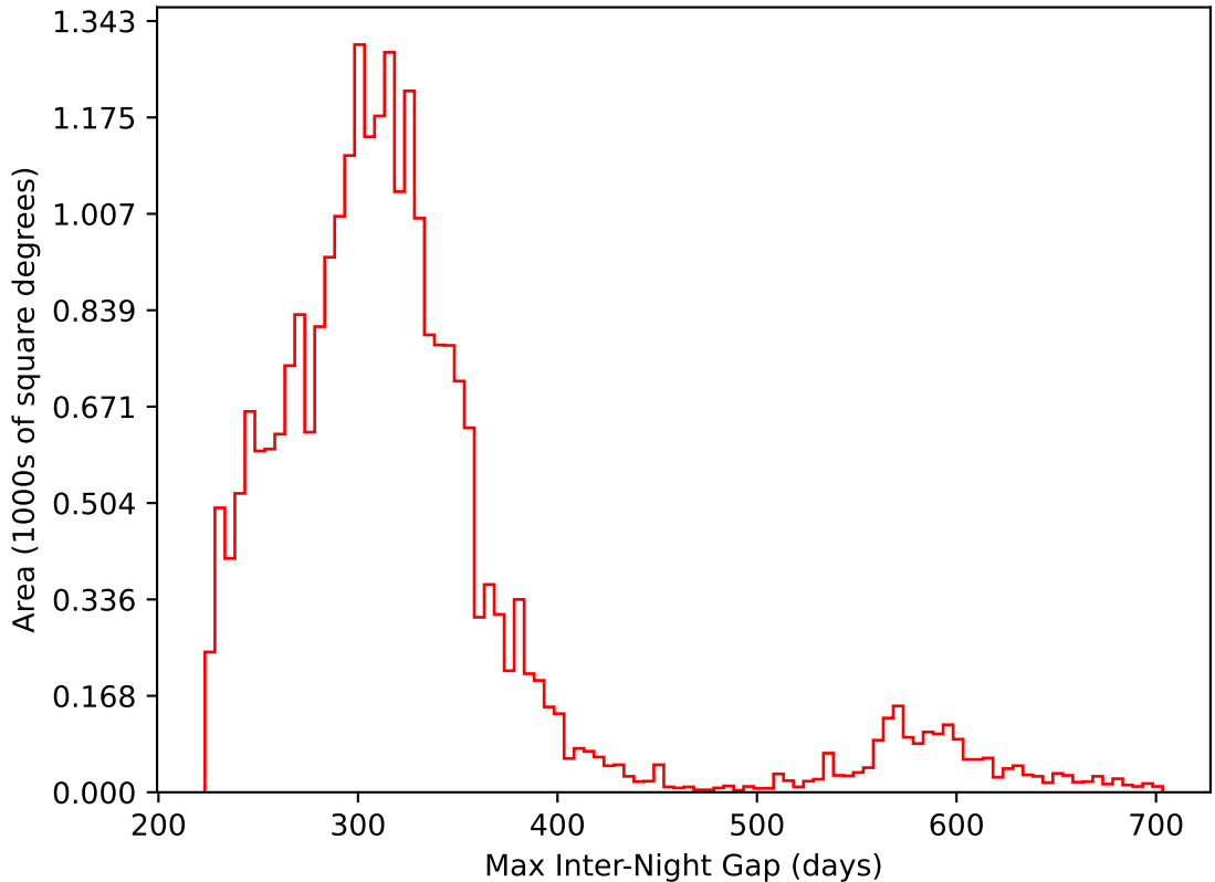
roll_uniform_eh_acc0.2_mjdp0_v3.4_10yrs All sky i band: Max Inter-Night Gap
