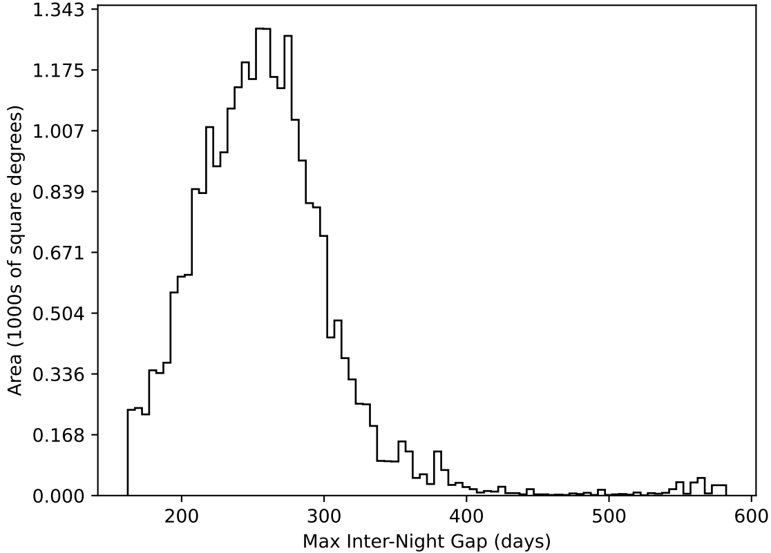
roll_uniform_eh_acc0.2_mjdp0_v3.4_10yrs All sky all bands: Max Inter-Night Gap
