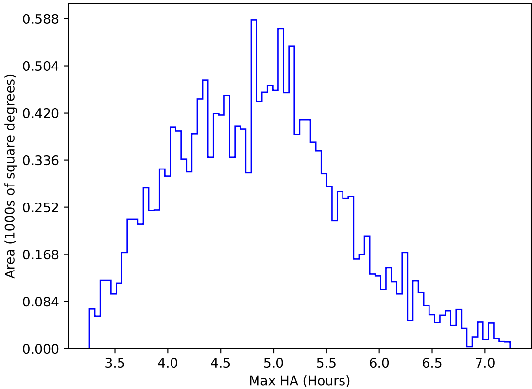
roll_uniform_eh_acc0.2_mjdp0_v3.4_10yrs WFD z band: Max HA
