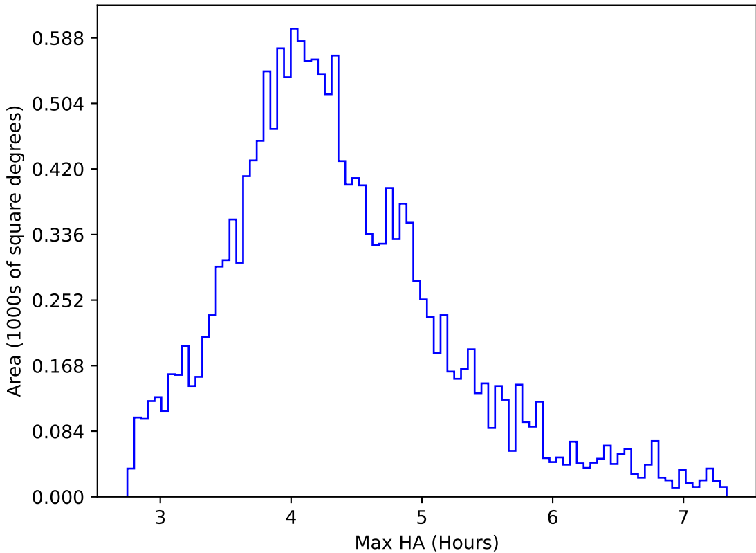
roll_uniform_eh_acc0.2_mjdp0_v3.4_10yrs WFD r band: Max HA
