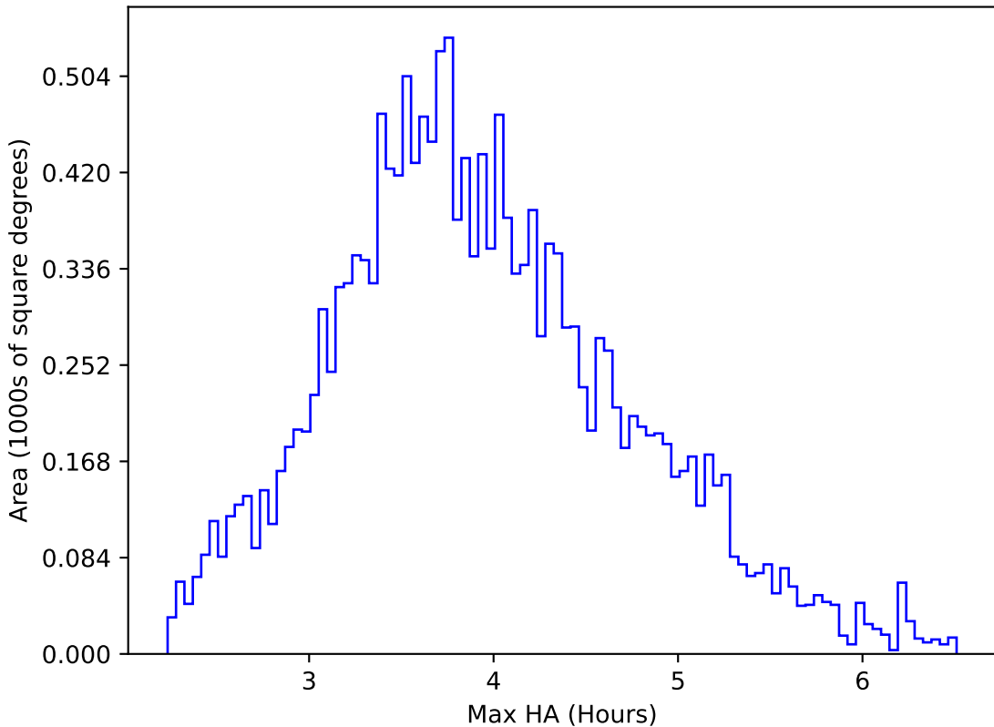
roll_uniform_eh_acc0.2_mjdp0_v3.4_10yrs WFD g band: Max HA
