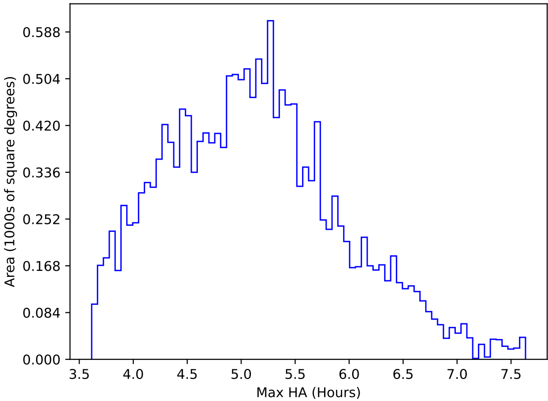
roll_uniform_eh_acc0.2_mjdp0_v3.4_10yrs WFD all bands: Max HA
