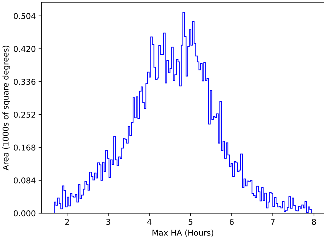
roll_uniform_eh_acc0.2_mjdp0_v3.4_10yrs All sky z band: Max HA
