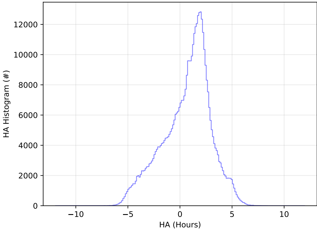
roll_uniform_eh_acc0.2_mjdp0_v3.4_10yrs WFD z band: HA Histogram
