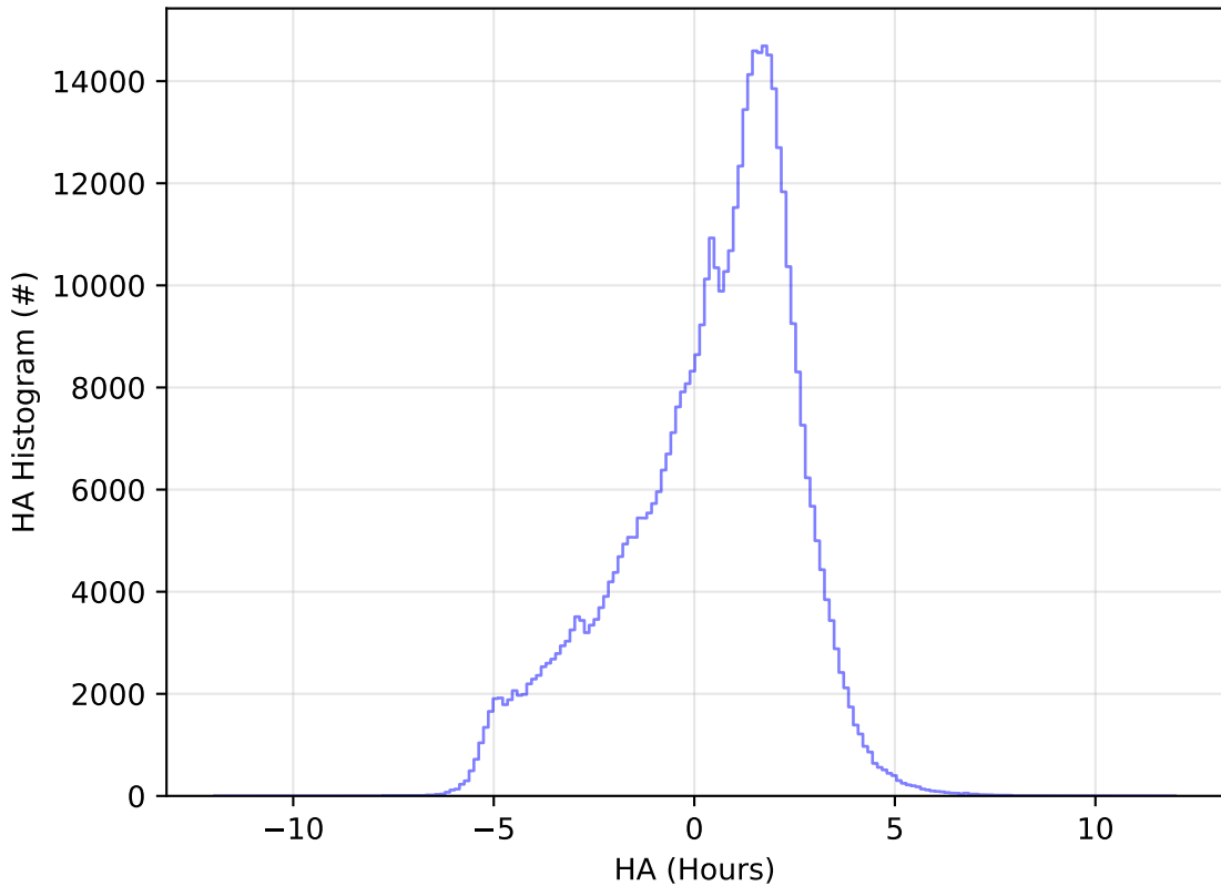
roll_uniform_eh_acc0.2_mjdp0_v3.4_10yrs WFD r band: HA Histogram
