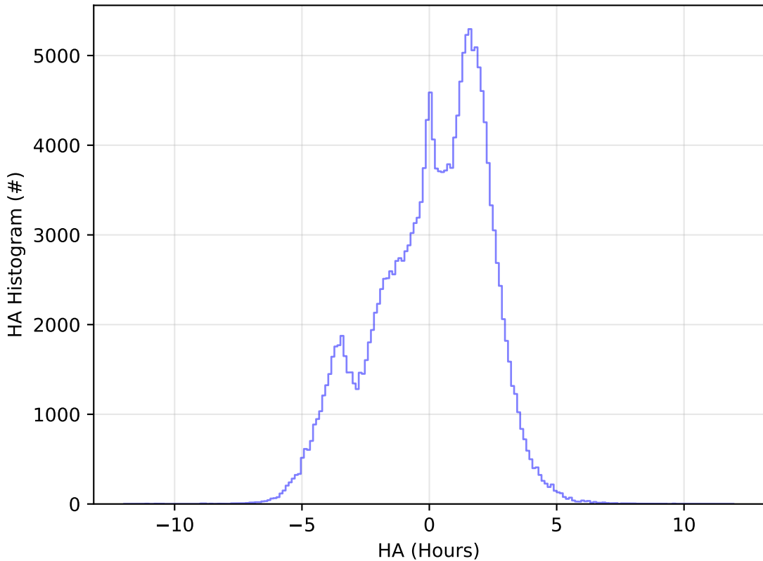
roll_uniform_eh_acc0.2_mjdp0_v3.4_10yrs WFD g band: HA Histogram
