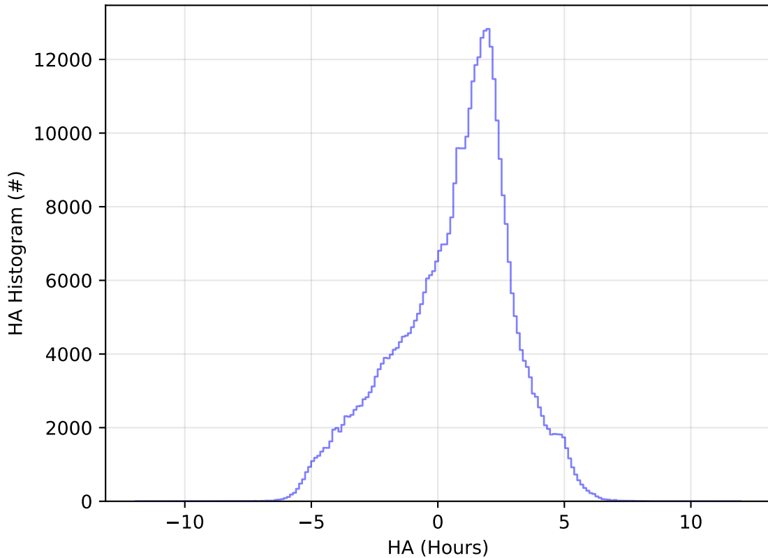
roll_uniform_eh_acc0.2_mjdp0_v3.4_10yrs All sky z band: HA Histogram
