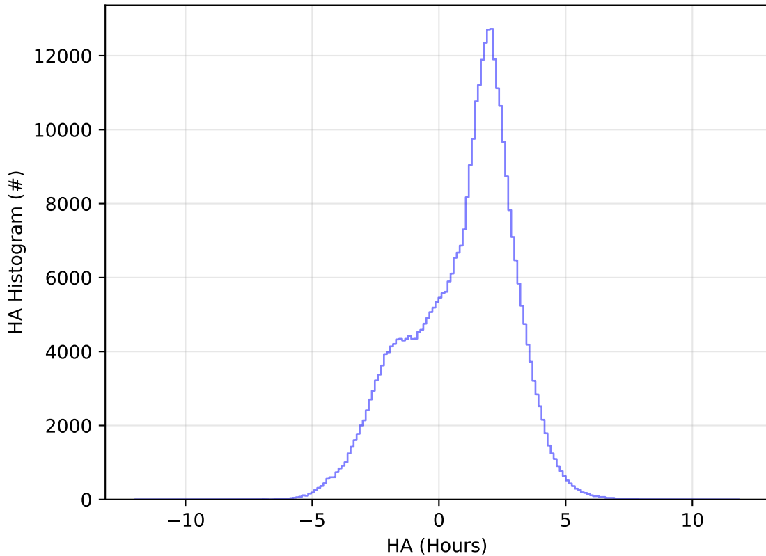
roll_uniform_eh_acc0.2_mjdp0_v3.4_10yrs All sky y band: HA Histogram
