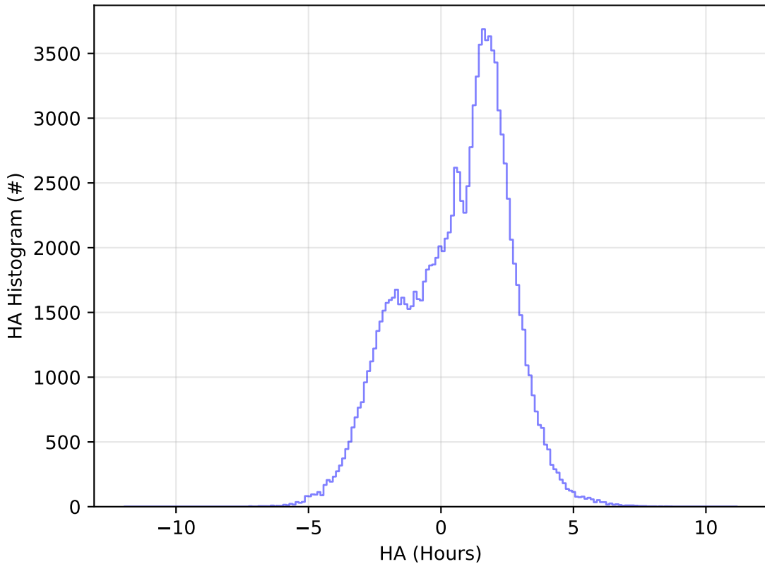
roll_uniform_eh_acc0.2_mjdp0_v3.4_10yrs All sky u band: HA Histogram
