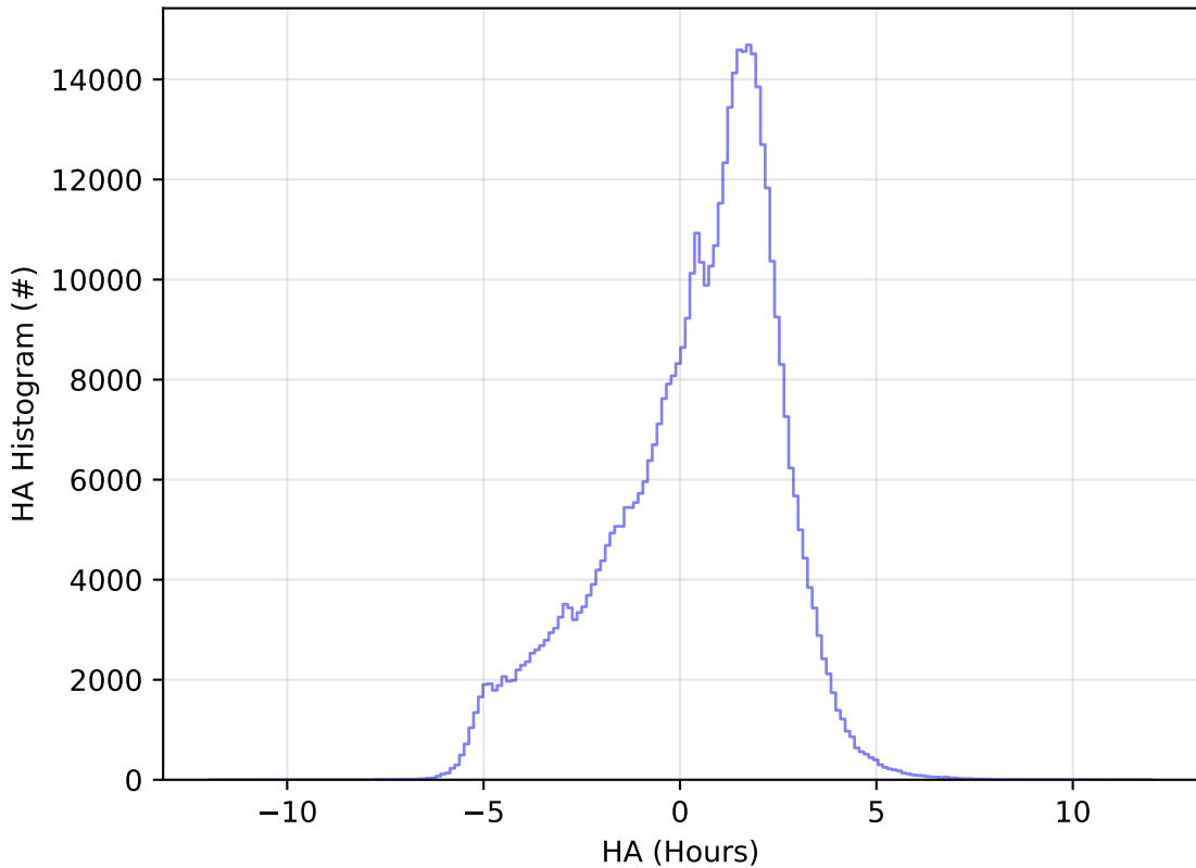
roll_uniform_eh_acc0.2_mjdp0_v3.4_10yrs All sky r band: HA Histogram
