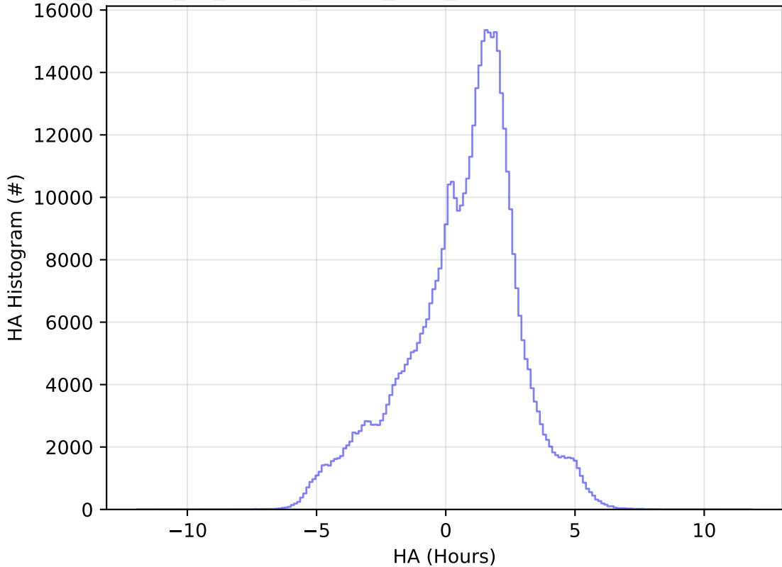
roll_uniform_eh_acc0.2_mjdp0_v3.4_10yrs All sky i band: HA Histogram
