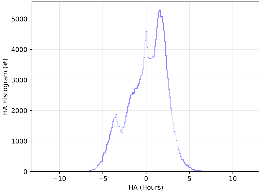
roll_uniform_eh_acc0.2_mjdp0_v3.4_10yrs All sky g band: HA Histogram
