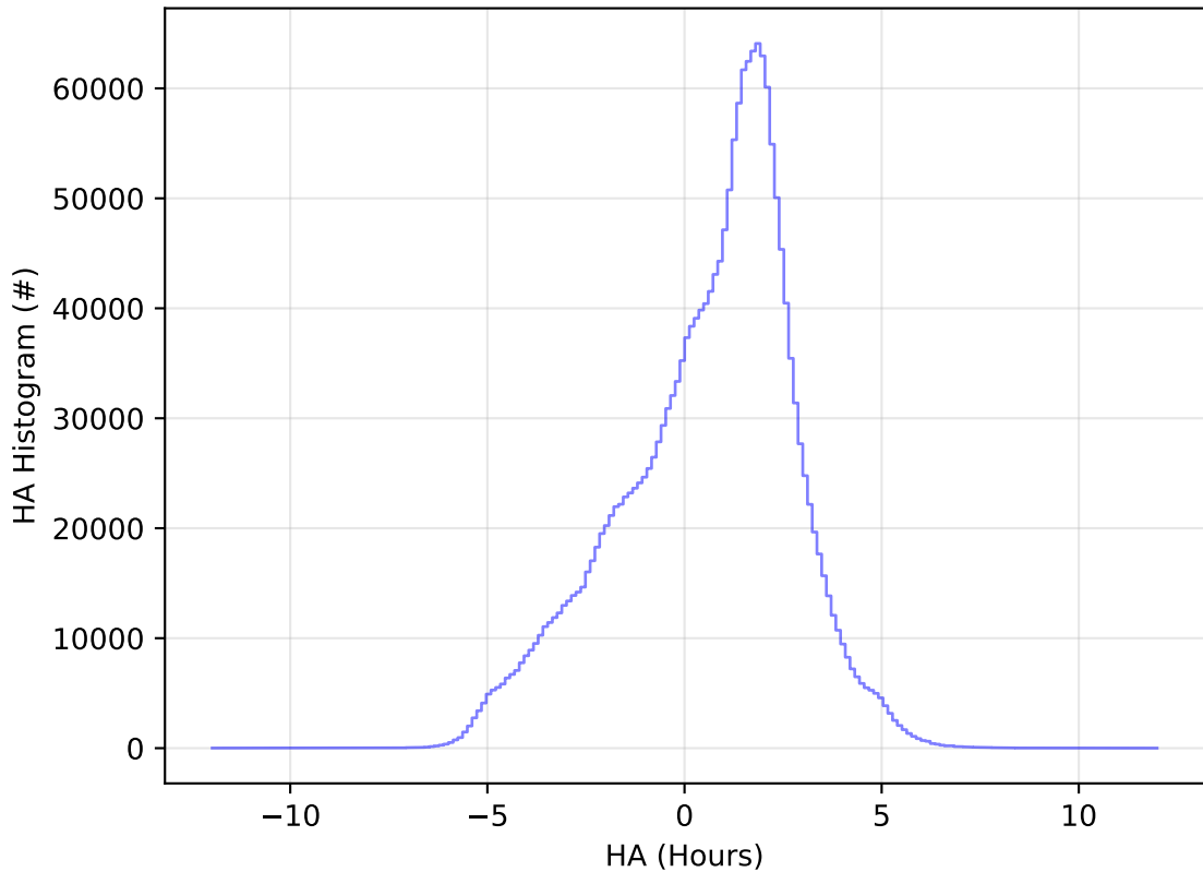
roll_uniform_eh_acc0.2_mjdp0_v3.4_10yrs All sky all bands: HA Histogram
