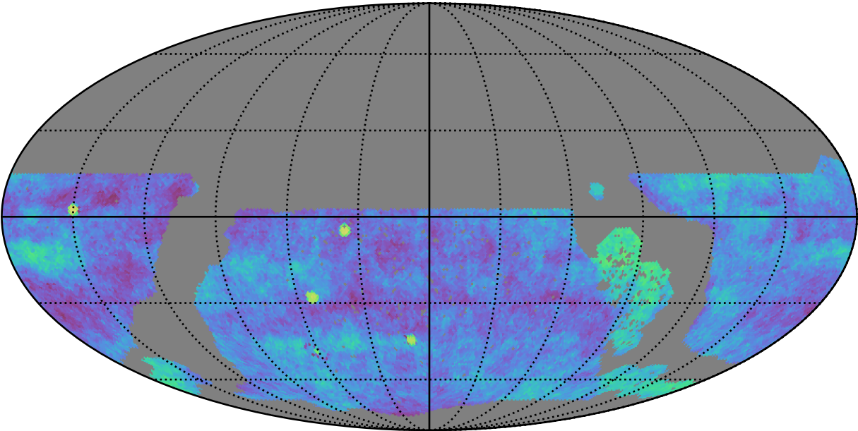
roll_uniform_eh_acc0.2_mjdp0_v3.4_10yrs gri WFD: Fraction of visits in pairs (20-90 min)
