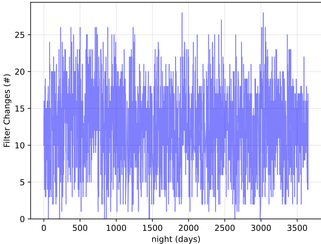
roll_uniform_eh_acc0.2_mjdp0_v3.4_10yrs Per Night: Filter Changes
