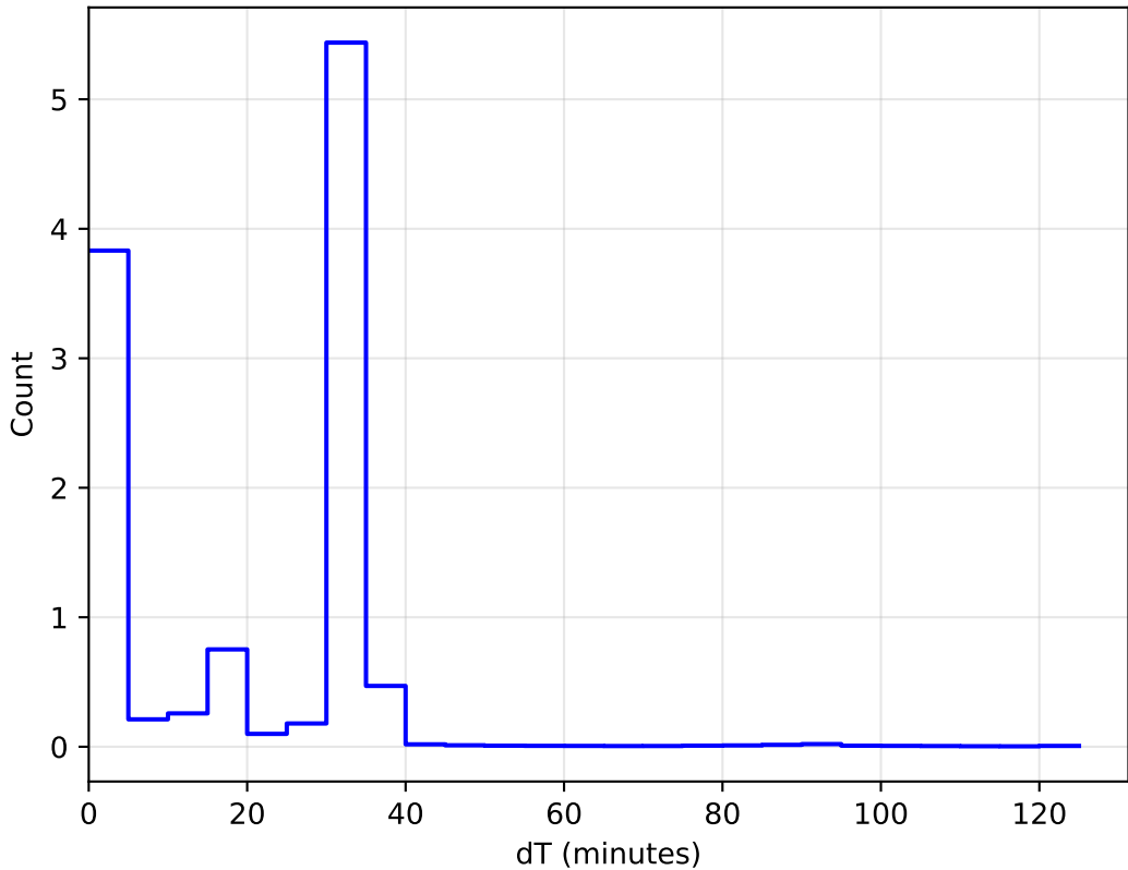
roll_uniform_eh_acc0.2_mjdp0_v3.4_10yrs WFD: DeltaT Histogram
