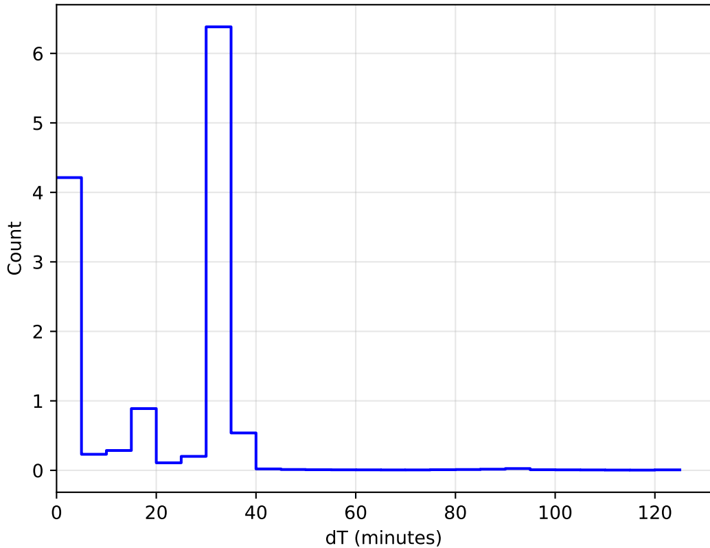
roll_uniform_eh_acc0.2_mjdp0_v3.4_10yrs All sky: DeltaT Histogram
