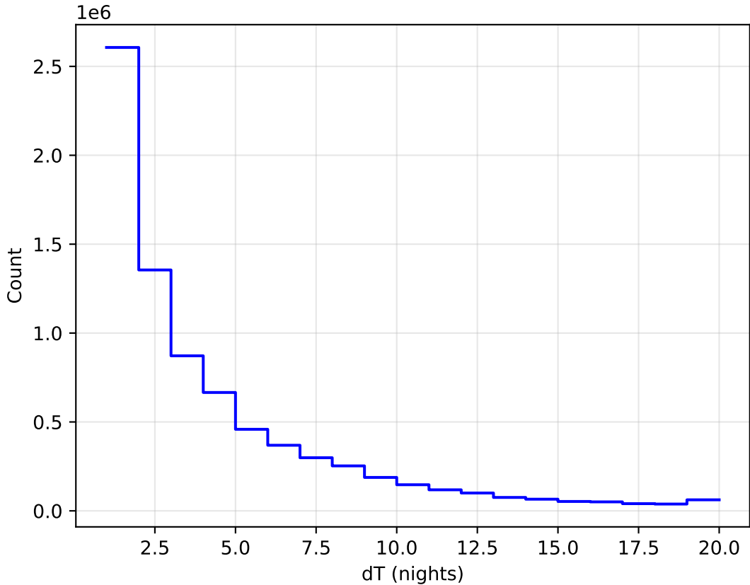
roll_uniform_eh_acc0.2_mjdp0_v3.4_10yrs WFD all bands: DeltaNight Histogram
