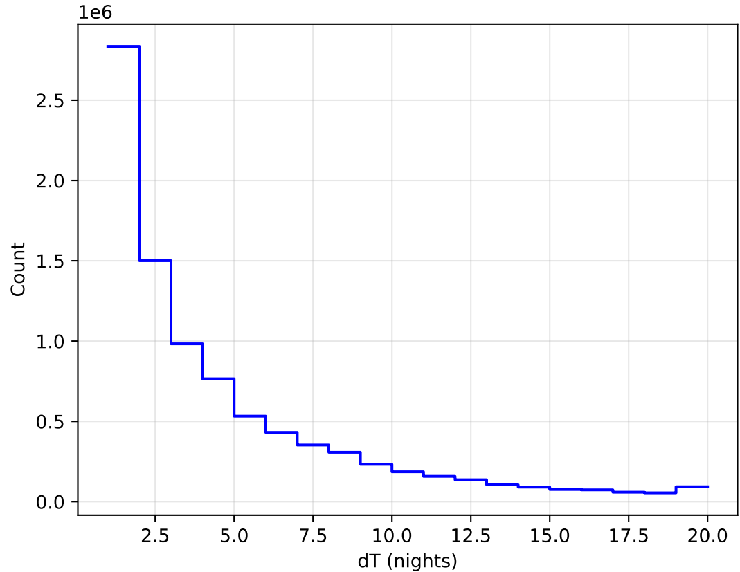
roll_uniform_eh_acc0.2_mjdp0_v3.4_10yrs All sky all bands: DeltaNight Histogram
