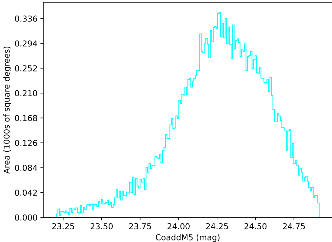
roll_uniform_eh_acc0.2_mjdp0_v3.4_10yrs Yr 1 u band: CoaddM5
