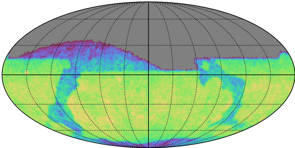
roll_uniform_eh_acc0.2_mjdp0_v3.4_10yrs Yr 1 i band: CoaddM5
