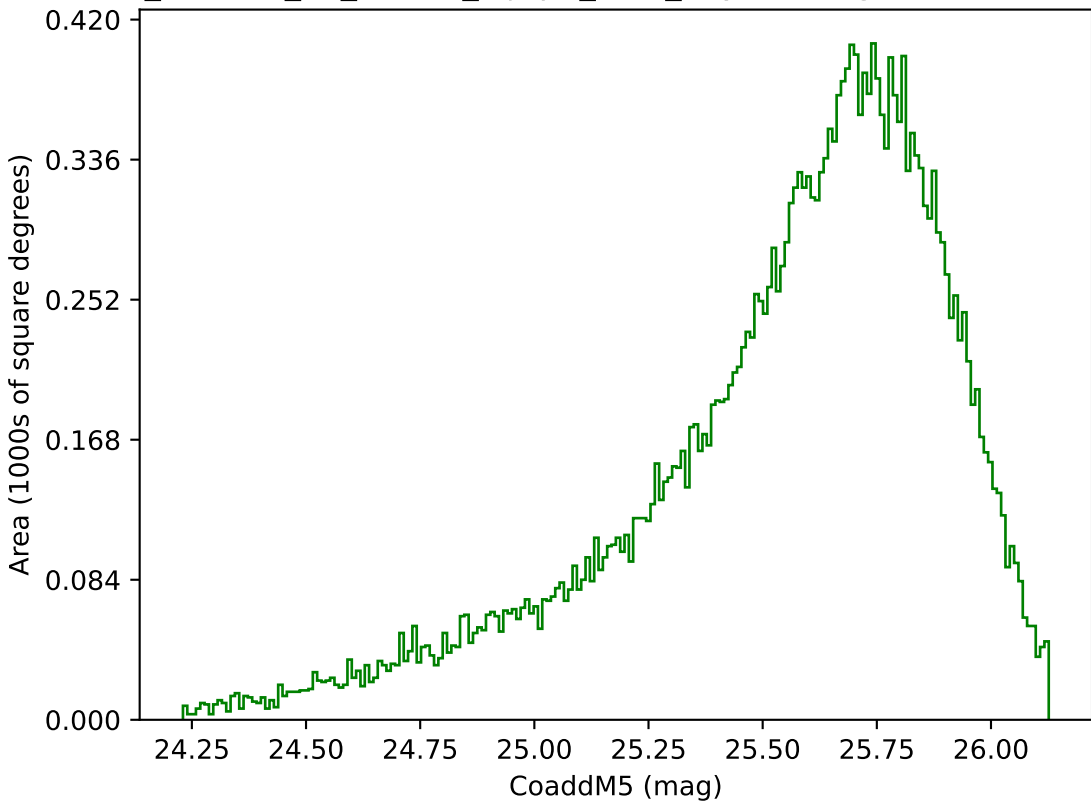
roll_uniform_eh_acc0.2_mjdp0_v3.4_10yrs Yr 1 g band: CoaddM5
