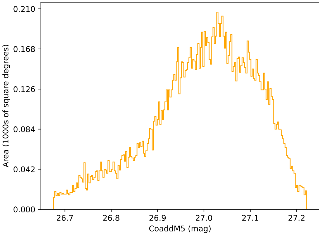
roll_uniform_eh_acc0.2_mjdp0_v3.4_10yrs WFD r band: CoaddM5
