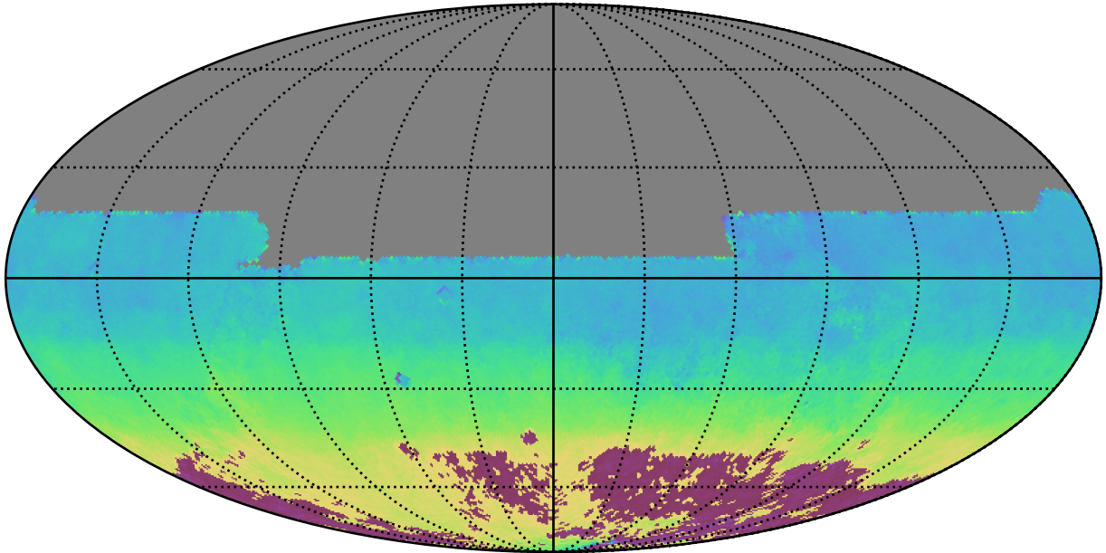
roll_uniform_eh_acc0.2_mjdp0_v3.4_10yrs All sky y band: AngleMean rotSkyPos
