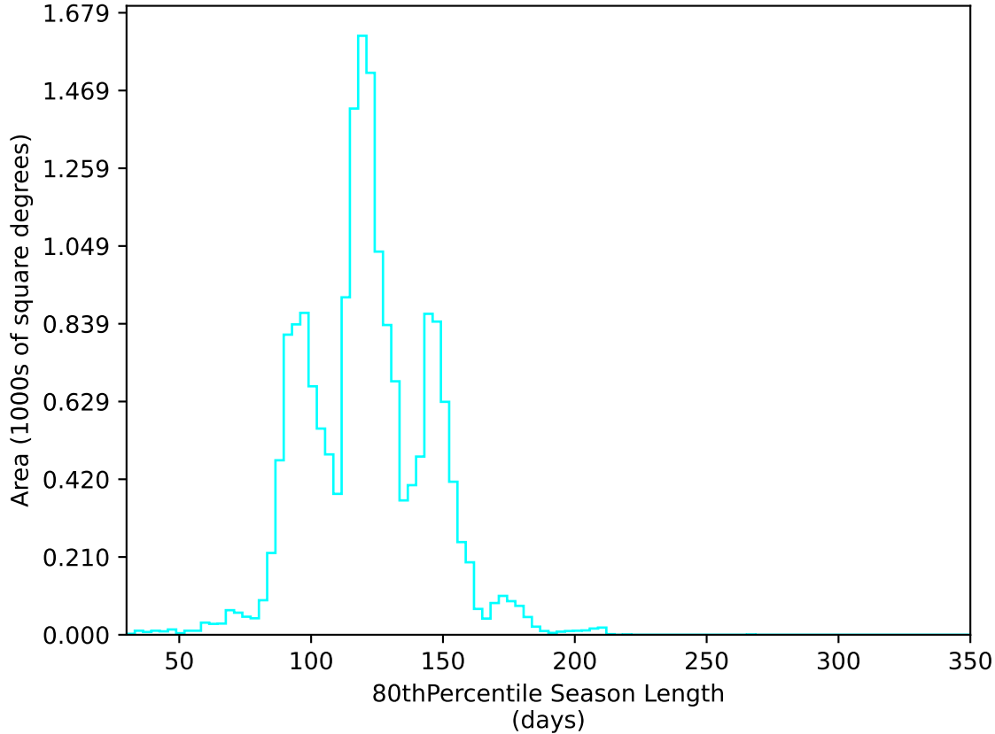
roll_uniform_eh_acc0.2_mjdp0_v3.4_10yrs WFD u band: 80thPercentile Season Length
