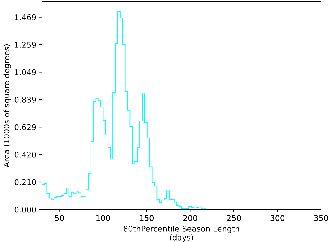
roll_uniform_eh_acc0.2_mjdp0_v3.4_10yrs All sky u band: 80thPercentile Season Length
