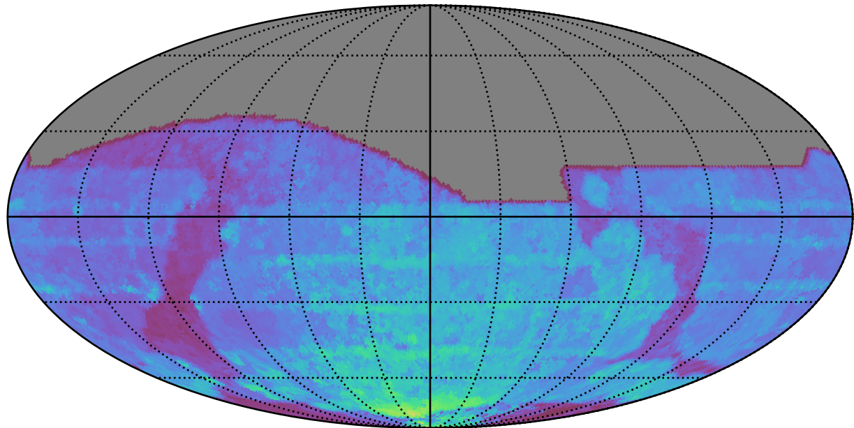
roll_uniform_eh_acc0.2_mjdp0_v3.4_10yrs All sky all bands: 80thPercentile Season Length
